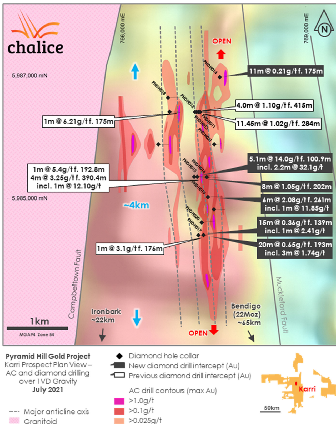
Figure 1. Karri Prospect Plan View – diamond and AC drilling results over 1VD gravity.
