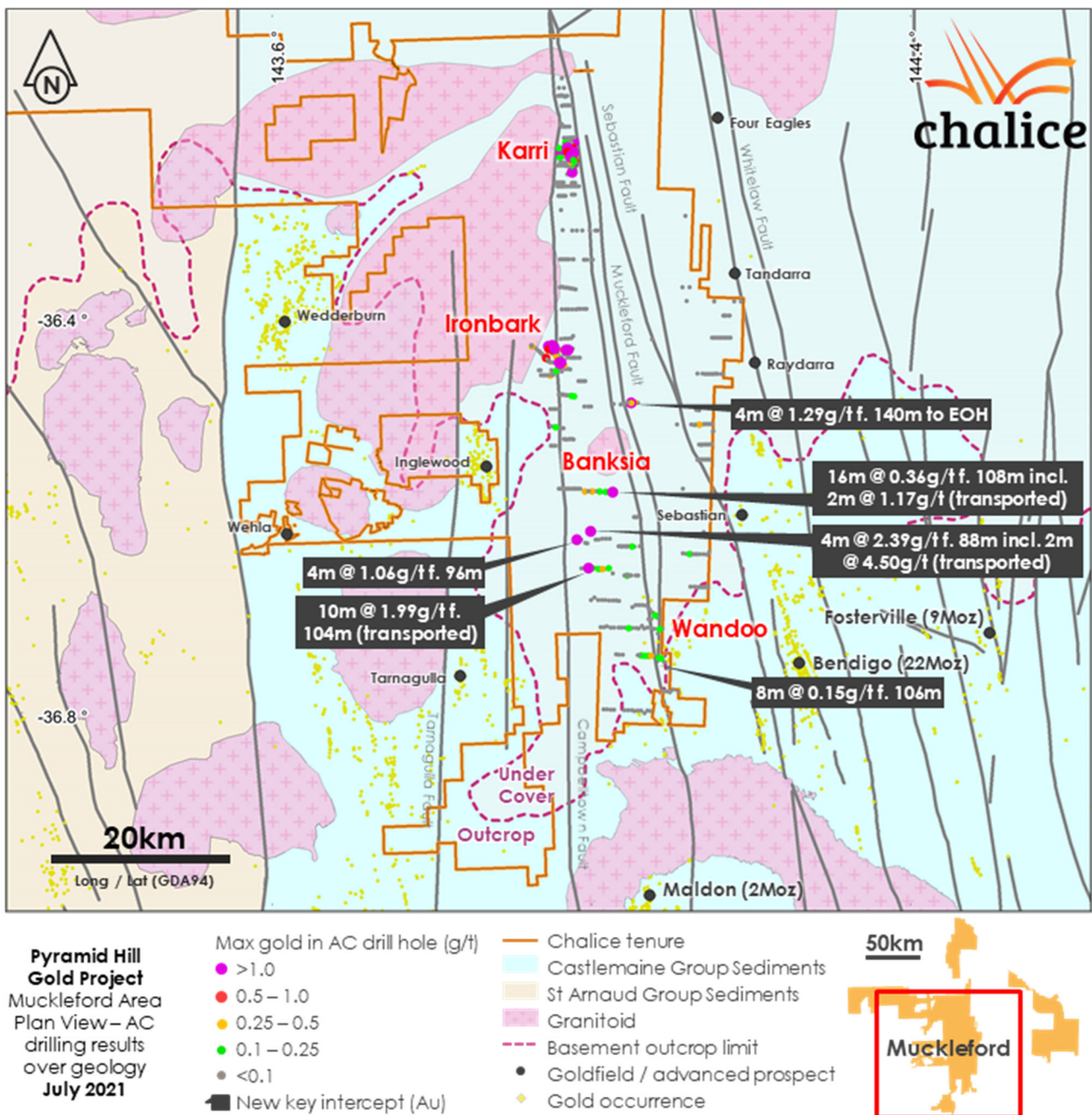
Figure 5. Muckleford Area Plan View – AC drilling results over geology
